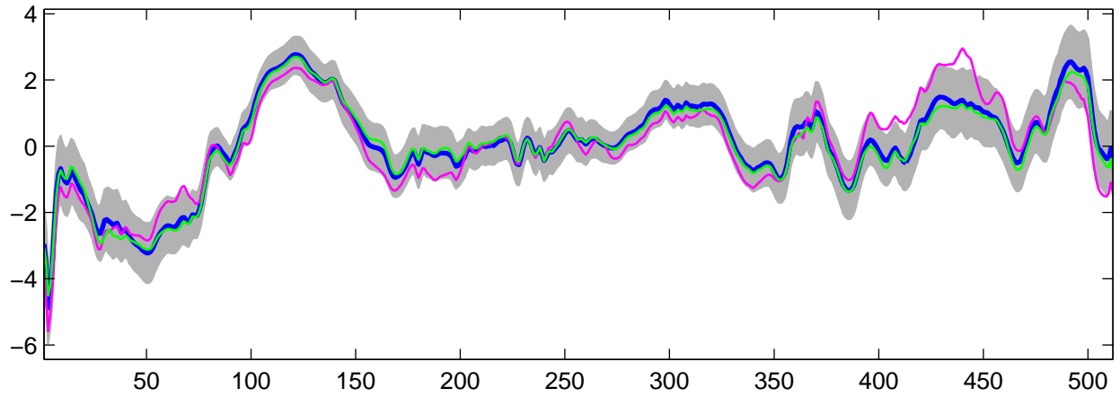
Estimated U_g(t) using G-WFMM: Normal data, run 8
