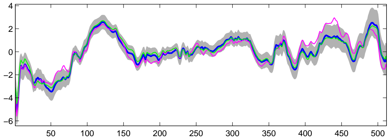
Estimated U_g(t) using R-WFMM: Normal data, run 8
