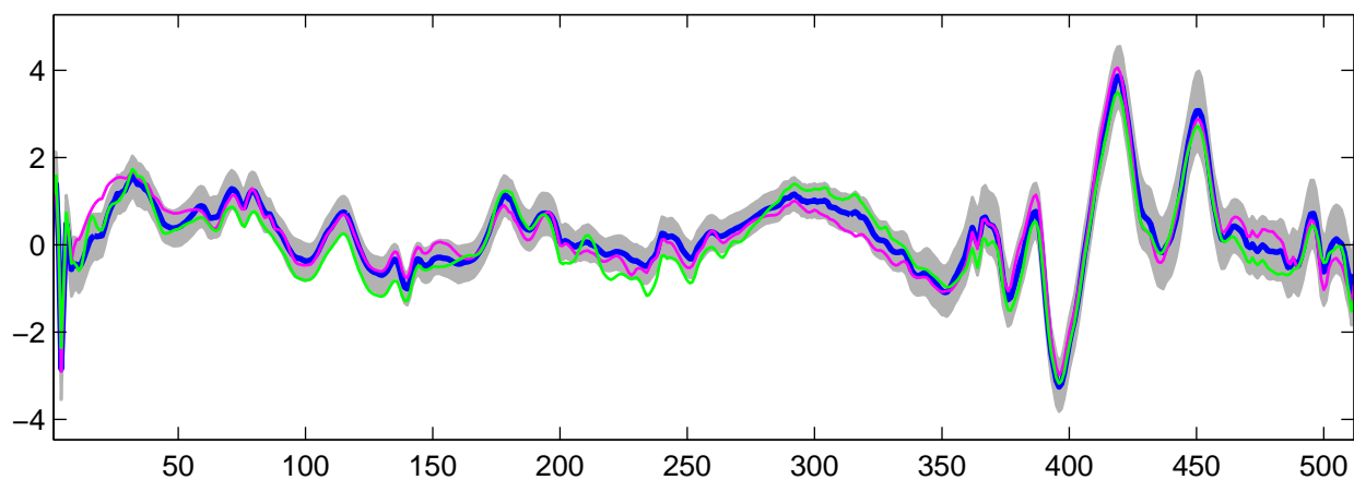
Estimated U_8(t) using R-WFMM: t_2 data, run 8
