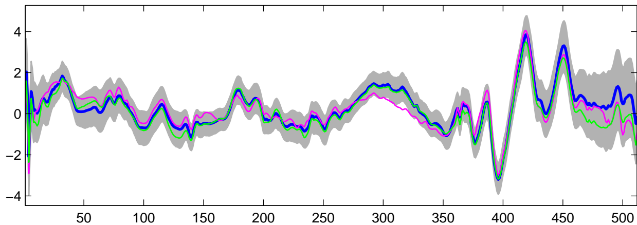
Estimated U_8(t) using G-WFMM: t_2 data, run 8
