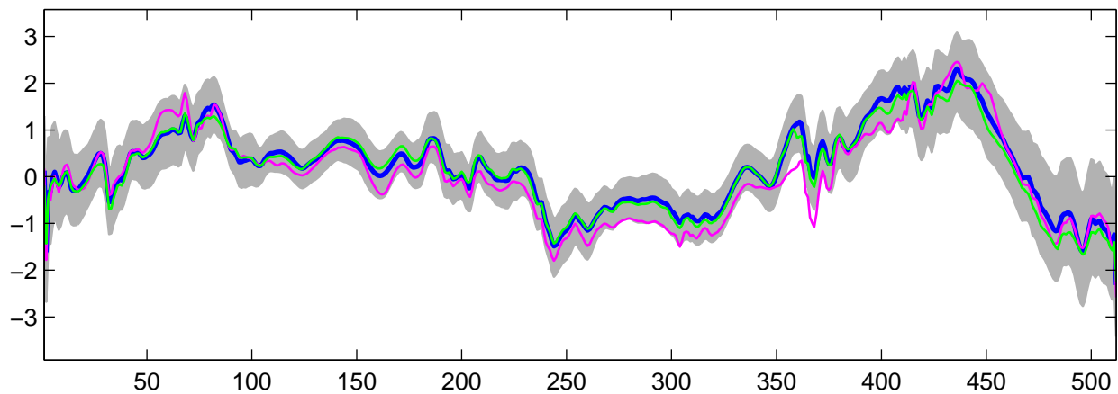
Estimated U_8(t) using G-WFMM: t_3 data, run 8
