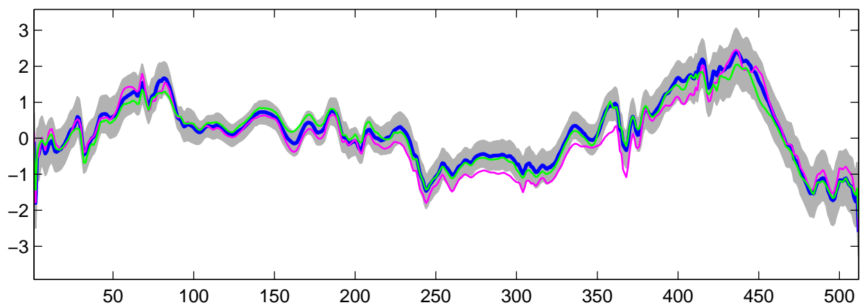
Estimated U_8(t) using R-WFMM: t_3 data, run 8
