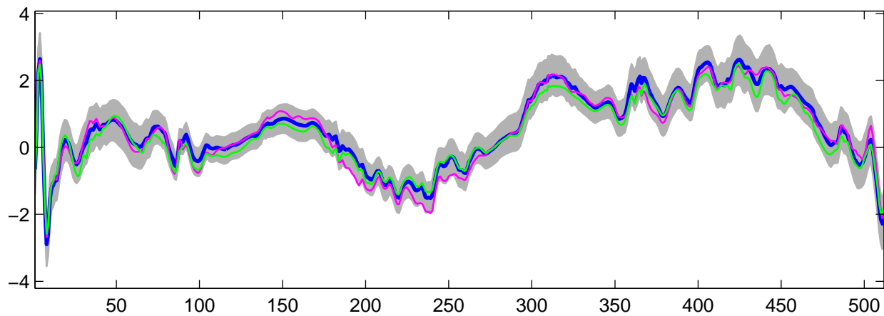
Estimated U_\theta(t) using R-WFMM: DE data, run 8
