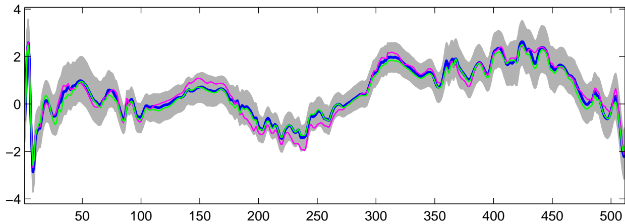
Estimated U_\theta(t) using G-WFMM: DE data, run 8
