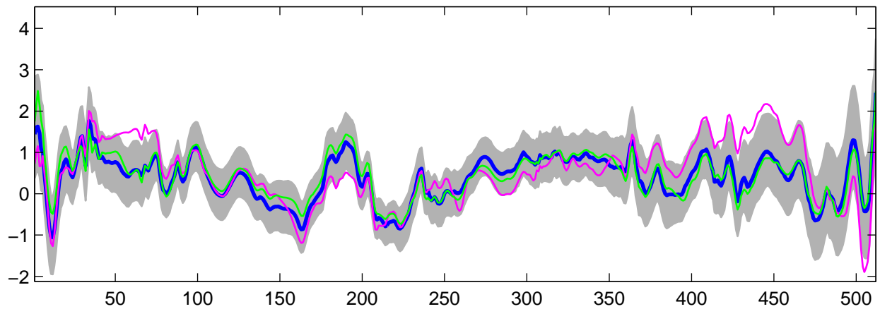
Estimated U_{\theta}(t) using R-WFMM: Normal data, run 8
