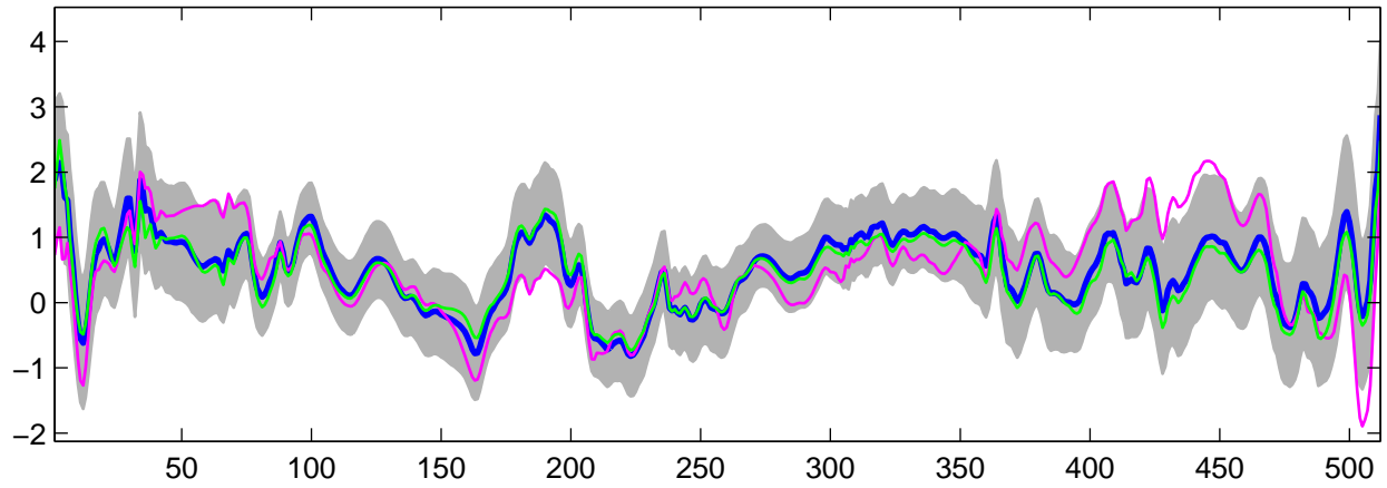
Estimated U_{\theta}(t) using G-WFMM: Normal data, run 8
