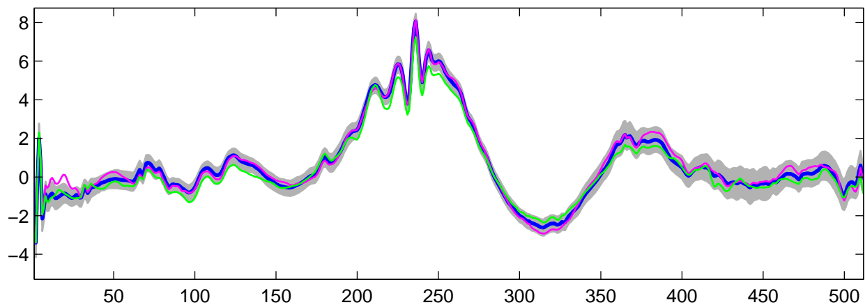
Estimated U_{\theta}(t) using R-WFMM: t_2 data, run 8
