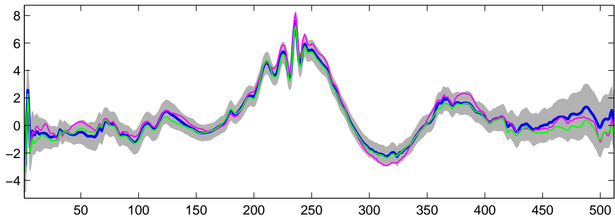
Estimated U_{\theta}(t) using G-WFMM: t_2 data, run 8
