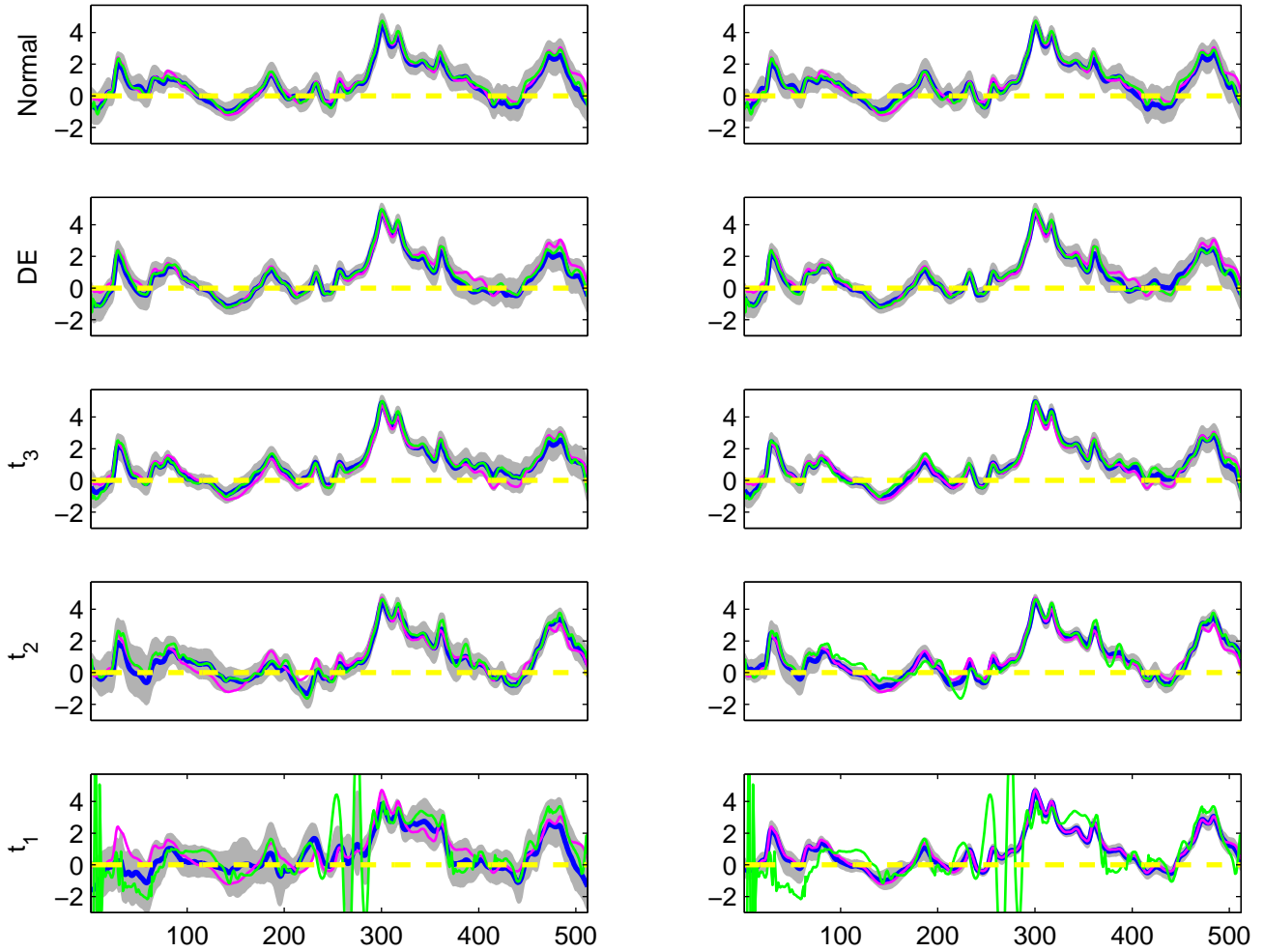
The estimated B_1(t) for 5 simulated datasets, simulation run 9 G-WFMM R-WFMM
