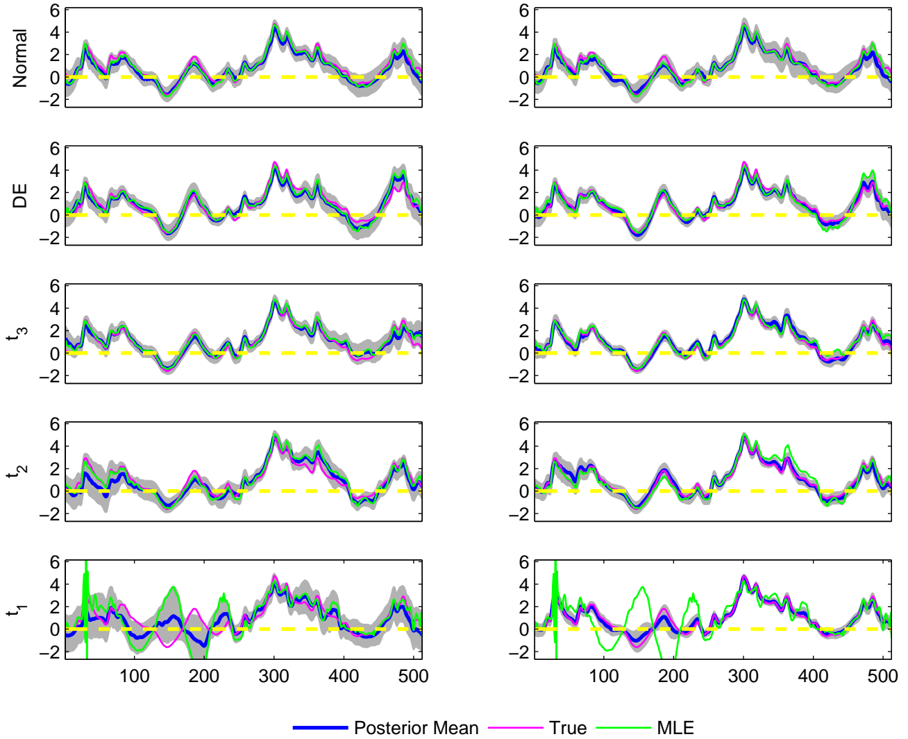
The estimated B_2(t) for 5 simulated datasets, simulation run 9 G-WFMM R-WFMM
