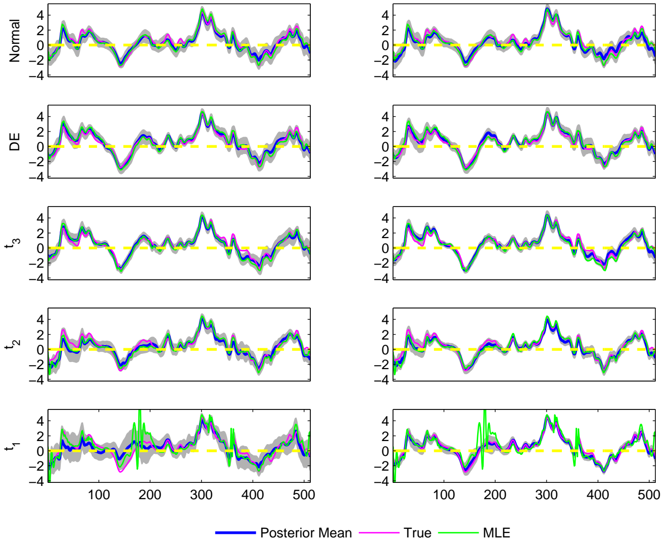
The estimated B_3(t) for 5 simulated datasets, simulation run 9
