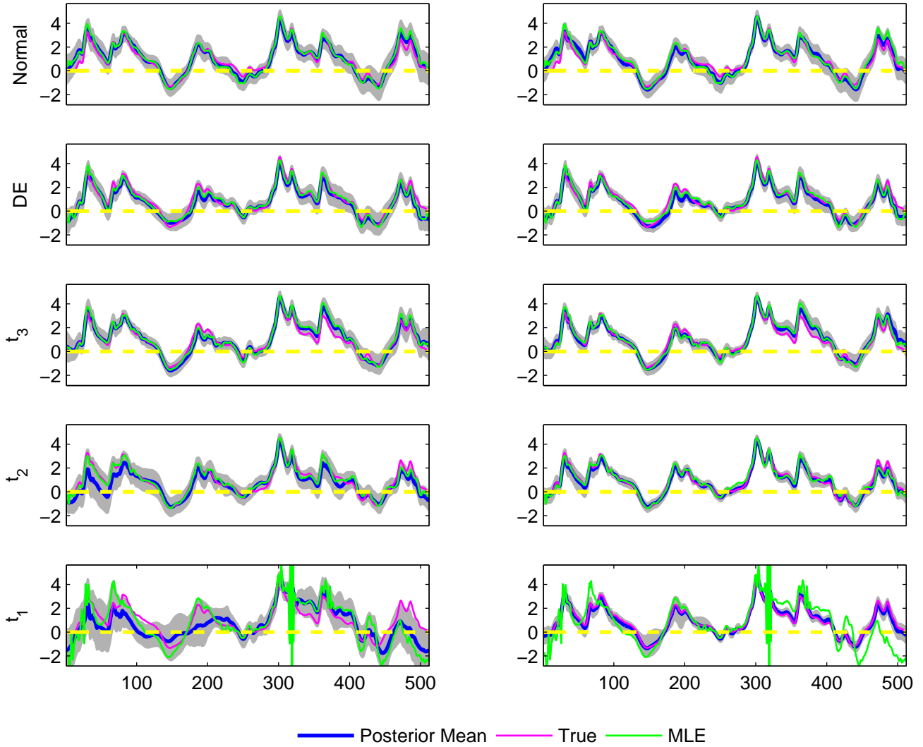
The estimated B_4(t) for 5 simulated datasets, simulation run 9 G-WFMM R-WFMM
