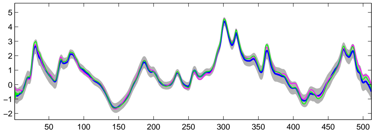
Estimated C_0(t) using G-WFMM: DE data, run 9
