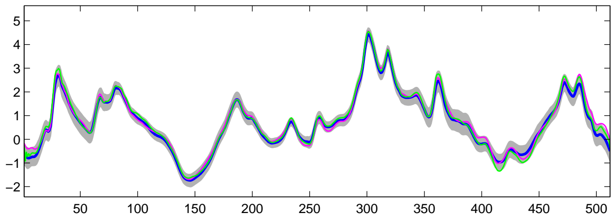
Estimated C_0(t) using R-WFMM: DE data, run 9
