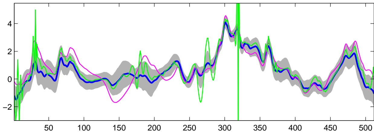
Estimated C_0(t) using G-WFMM: t_1 data, run 9
