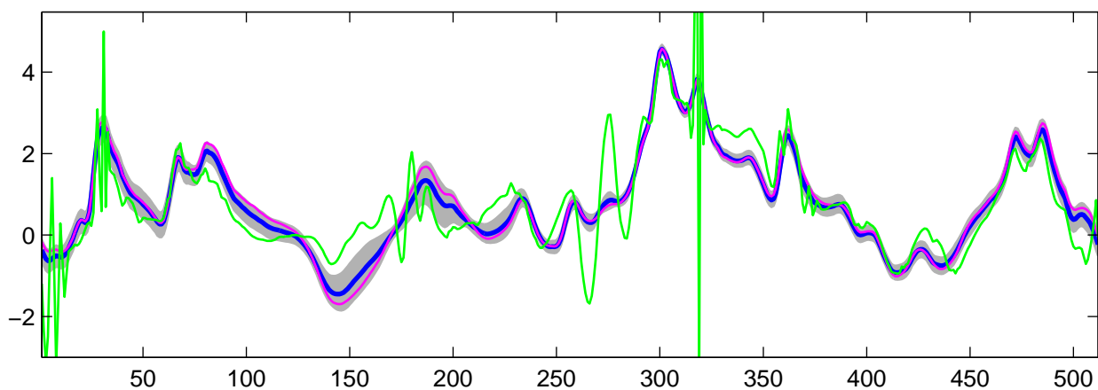
Estimated C_0(t) using R-WFMM: t_1 data, run 9
