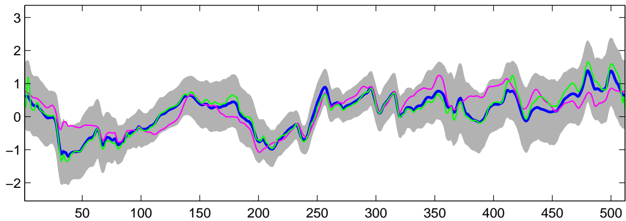
Estimated C_1(t) using G-WFMM: DE data, run 9
