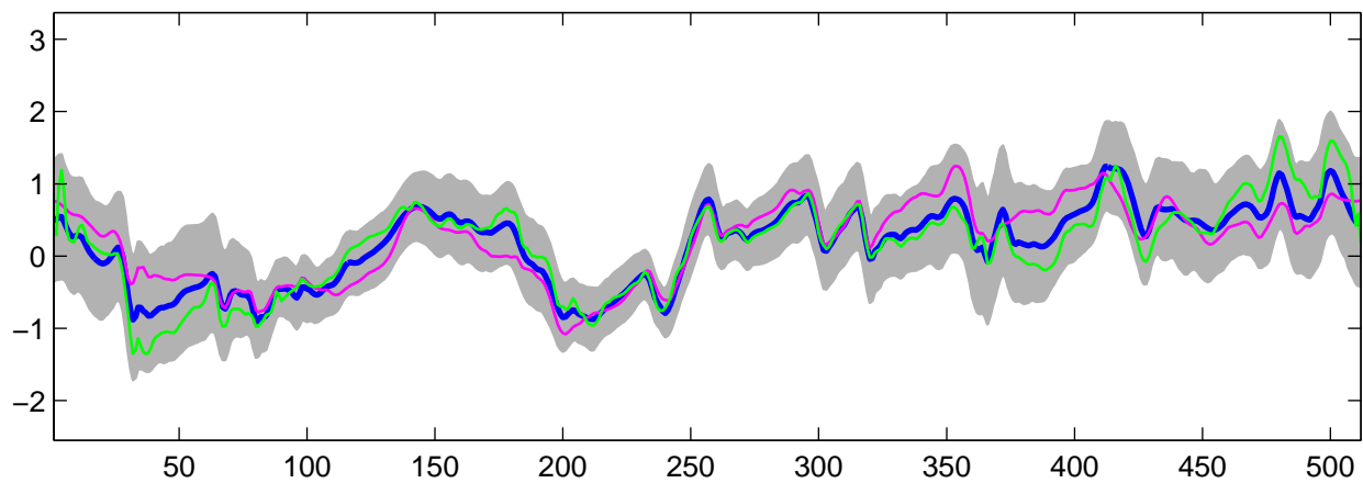
Estimated C_1(t) using R-WFMM: DE data, run 9
