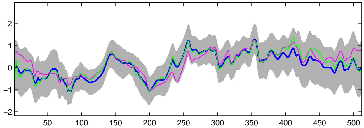
Estimated C_1(t) using G-WFMM: Normal data, run 9
