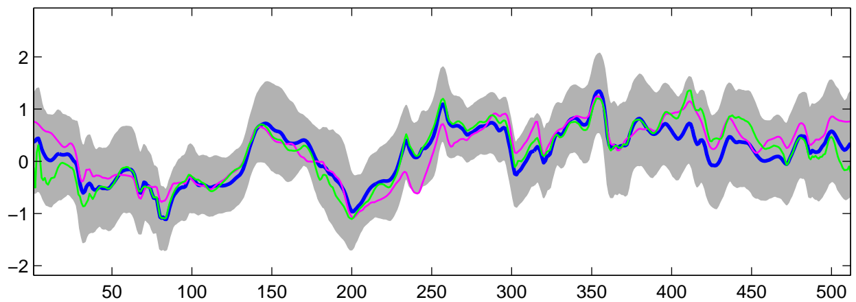
Estimated C_1(t) using R-WFMM: Normal data, run 9
