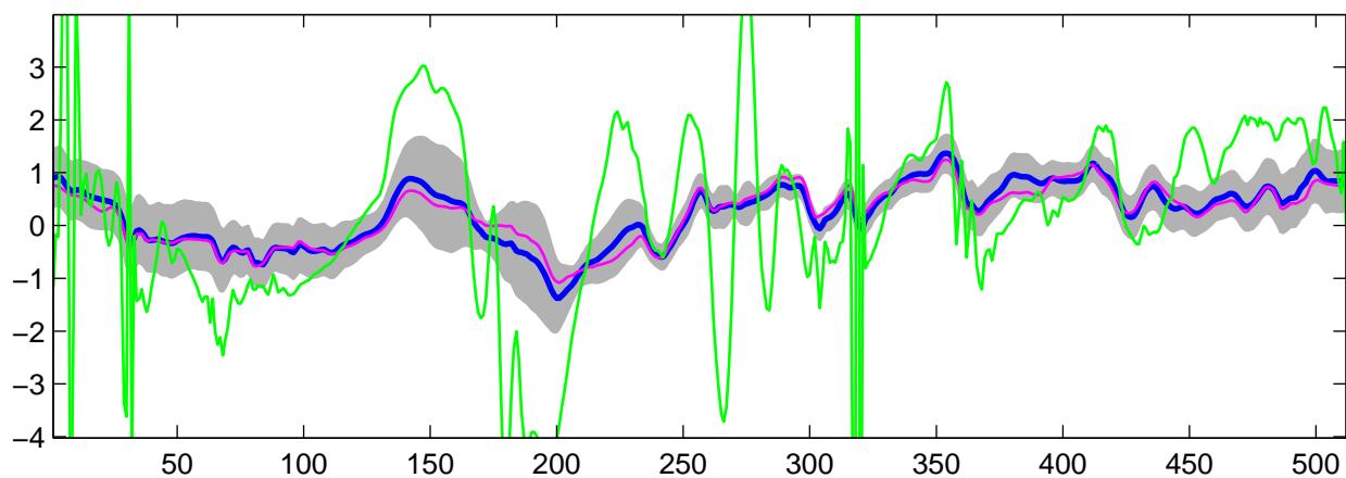
Estimated C_1(t) using R-WFMM: t_1 data, run 9
