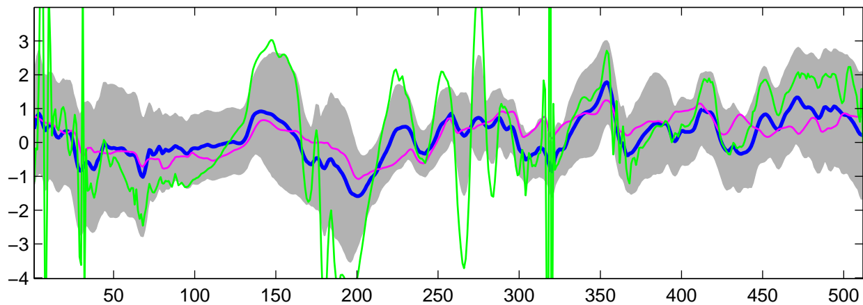
Estimated C_1(t) using G-WFMM: t_1 data, run 9
