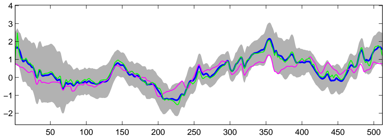
Estimated C_1(t) using G-WFMM: t_2 data, run 9
