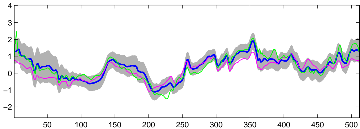
Estimated C_1(t) using R-WFMM: t_2 data, run 9
