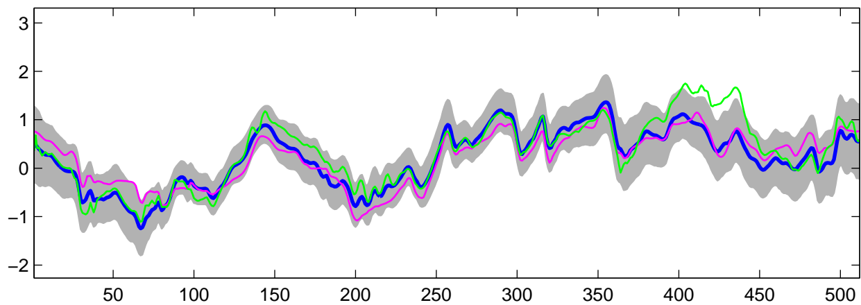
Estimated C_1(t) using R-WFMM: t_3 data, run 9
