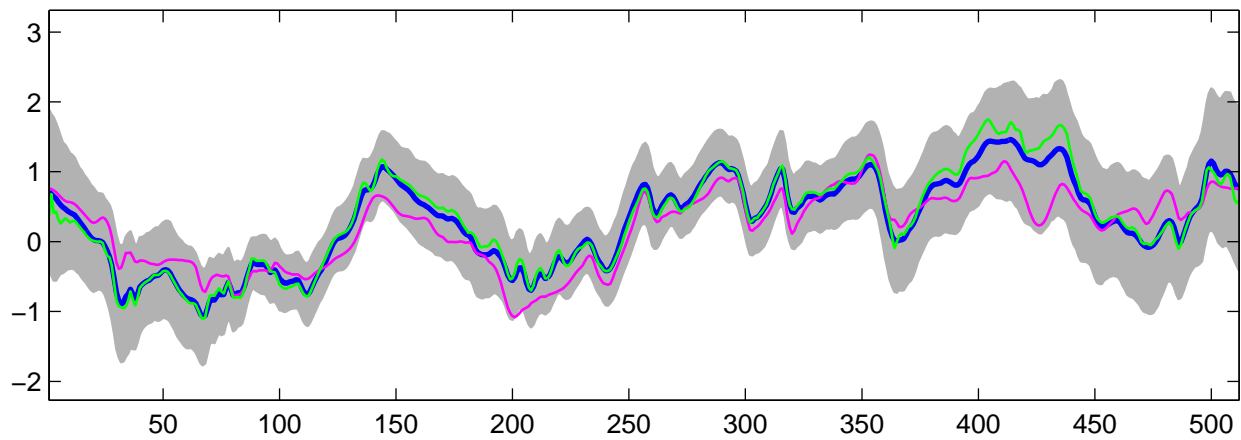
Estimated C_1(t) using G-WFMM: t_3 data, run 9
