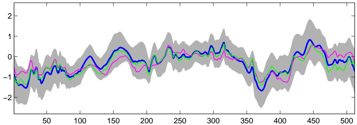
Estimated C_2(t) using R-WFMM: Normal data, run 9
