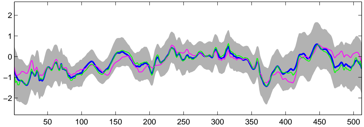
Estimated C_2(t) using G-WFMM: Normal data, run 9
