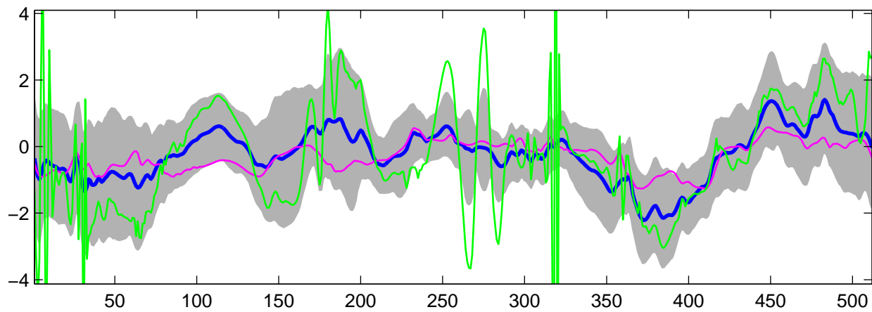
Estimated C_2(t) using G-WFMM: t_1 data, run 9
