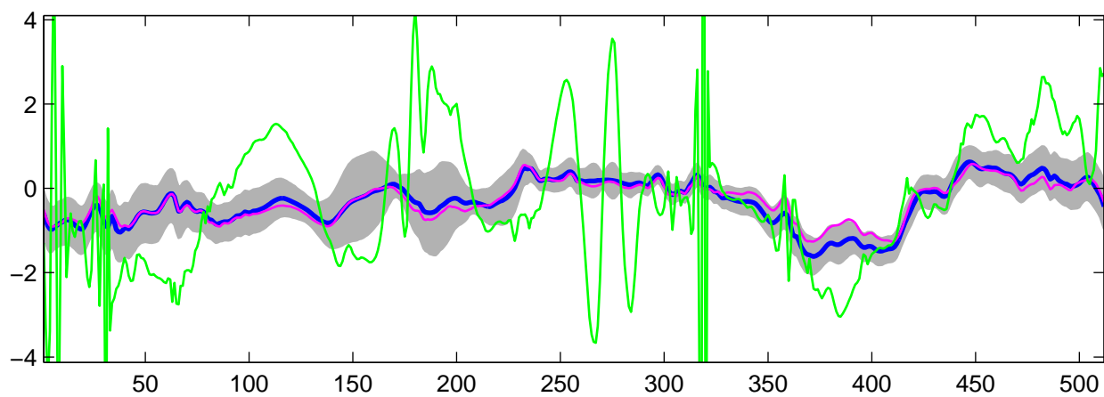
Estimated C_2(t) using R-WFMM: t_1 data, run 9
