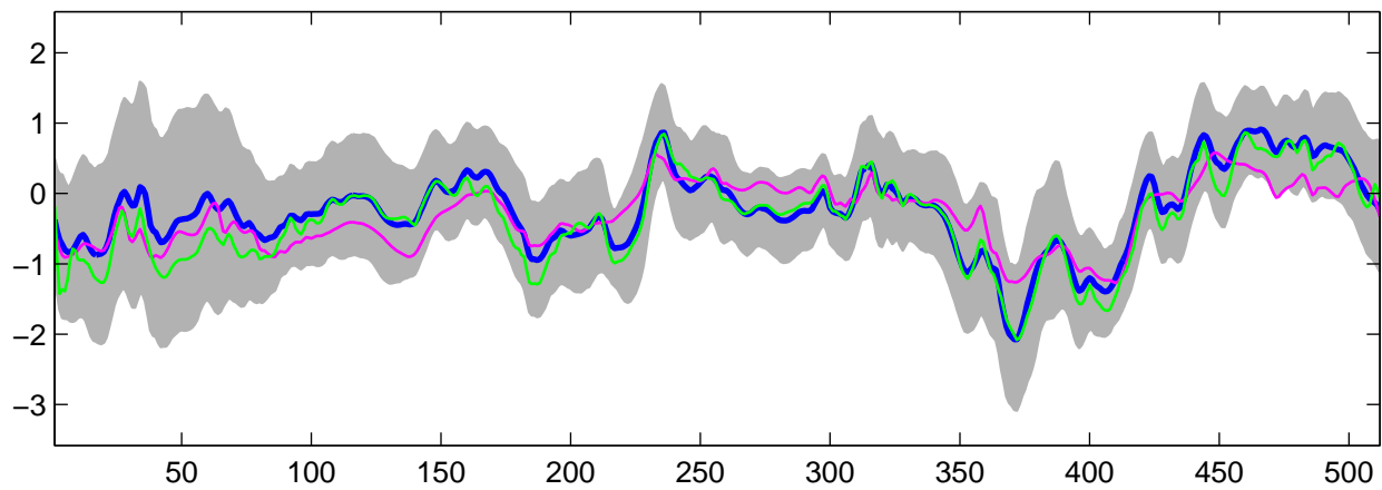
Estimated C_2(t) using G-WFMM: t_2 data, run 9
