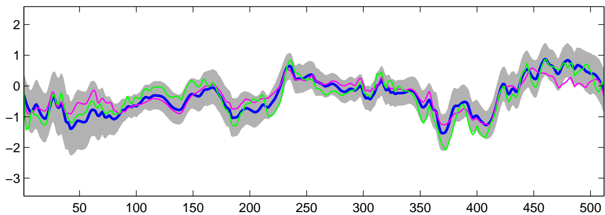
Estimated C_2(t) using R-WFMM: t_2 data, run 9
