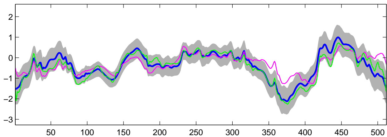
Estimated C_2(t) using R-WFMM: t_3 data, run 9
