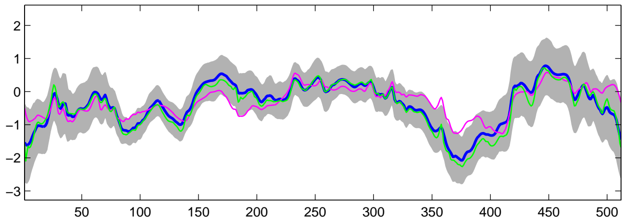
Estimated C_2(t) using G-WFMM: t_3 data, run 9
