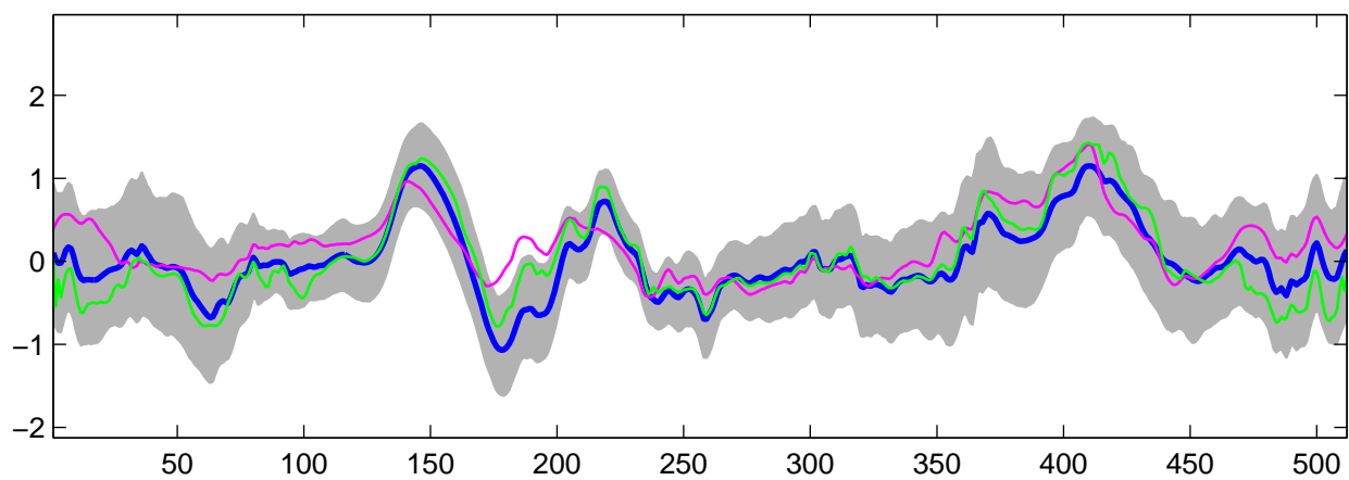
Estimated C_3(t) using R-WFMM: DE data, run 9
