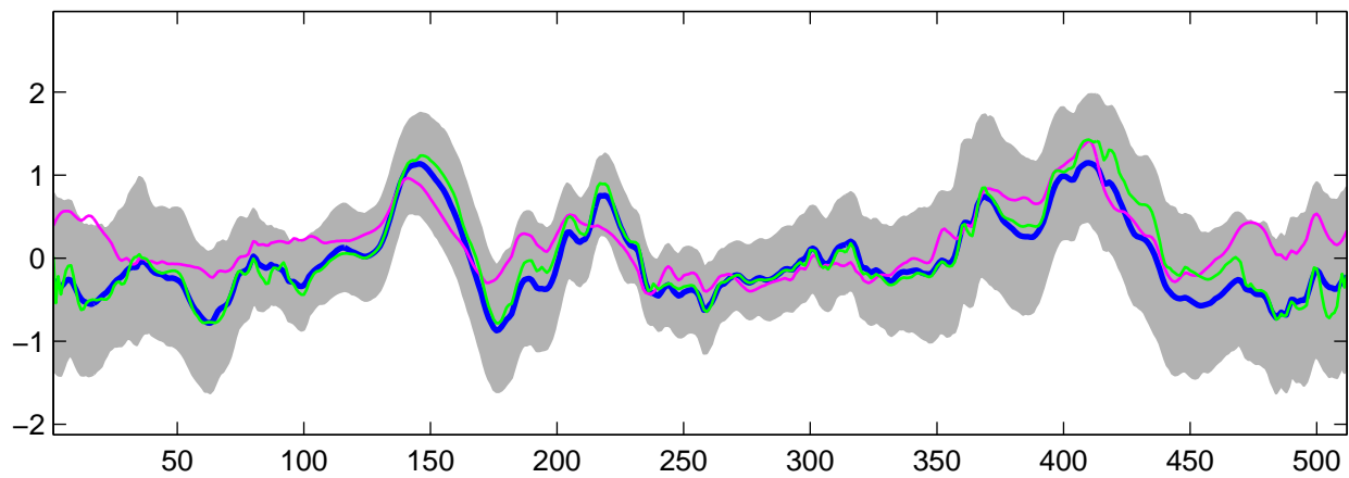
Estimated C_3(t) using G-WFMM: DE data, run 9
