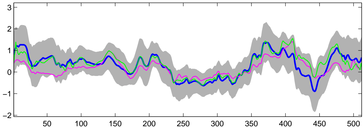
Estimated C_3(t) using R-WFMM: Normal data, run 9
