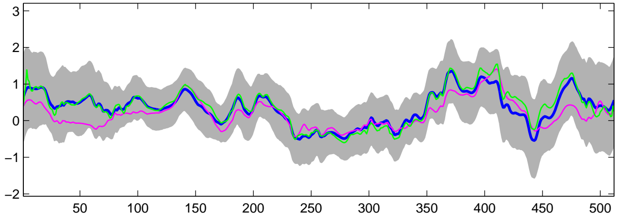
Estimated C_3(t) using G-WFMM: Normal data, run 9
