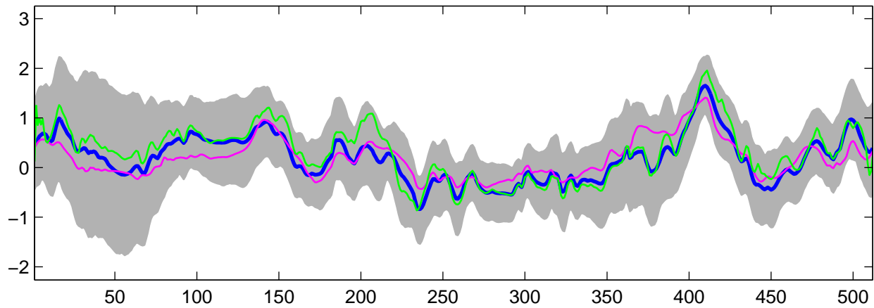
Estimated C_3(t) using G-WFMM: t_2 data, run 9
