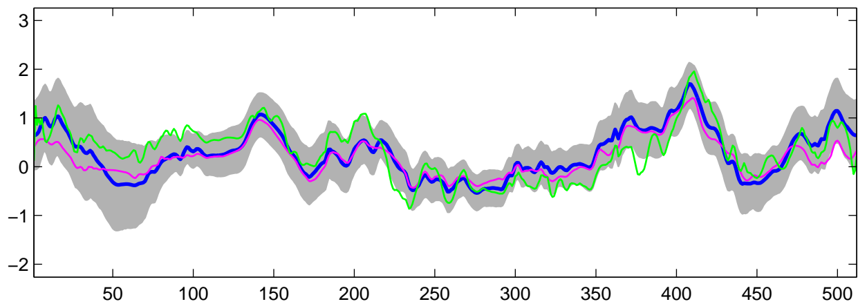
Estimated C_3(t) using R-WFMM: t_2 data, run 9
