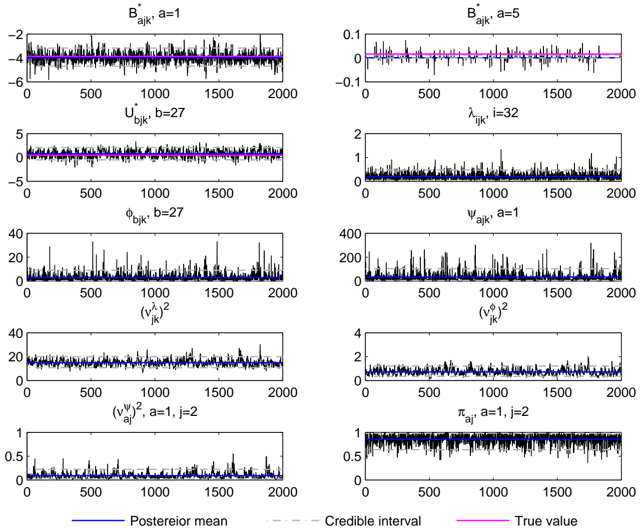
Trace plot, j=2, k=2 , Normal data, simulation run 9
