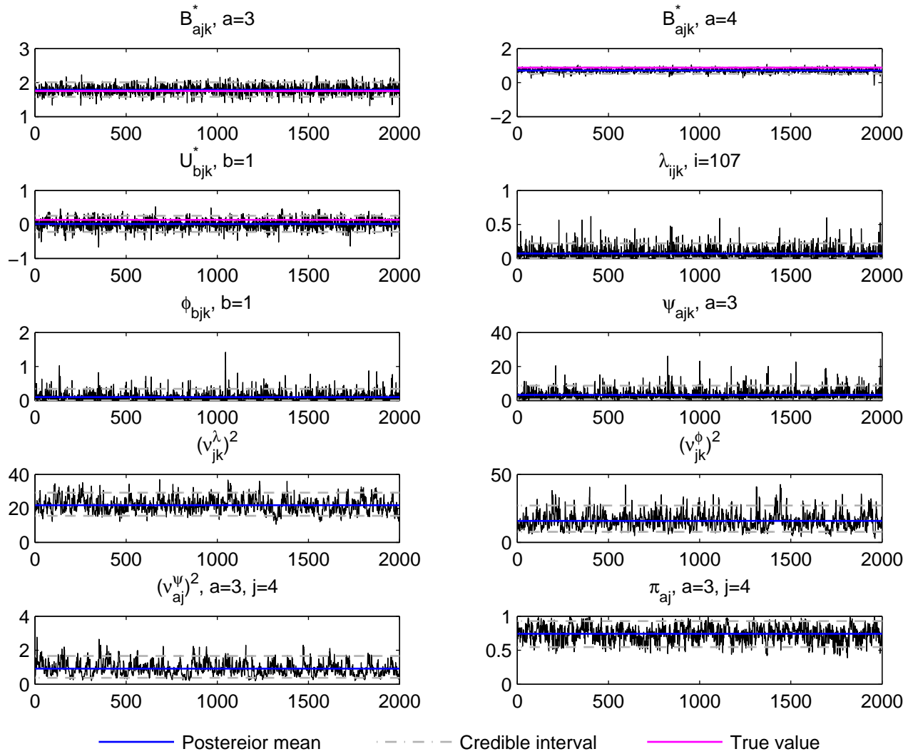
Trace plot, j=4, k=3, t_2 data, simulation run 9
