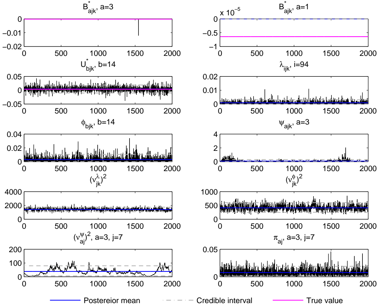
Trace plot, j=7, k=2, t_3 data, simulation run 9
