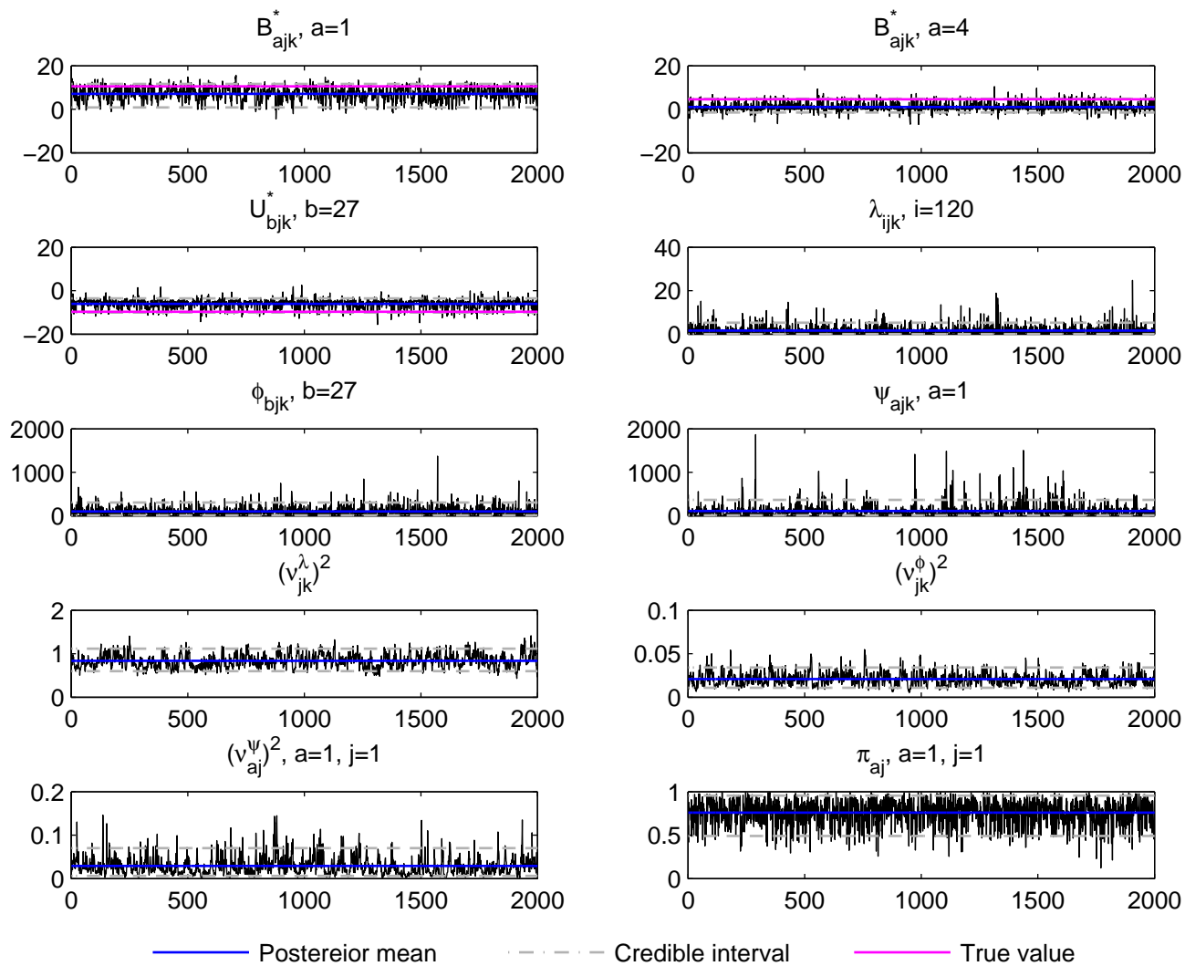
Trace plot, j=1, k=4 , DE data, simulation run 9
