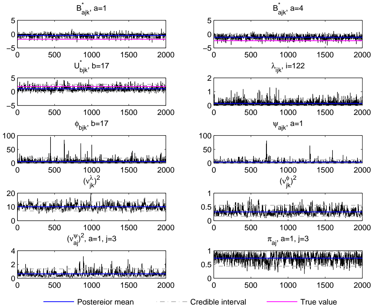
Trace plot, j=3, k=3 , Normal data, simulation run 9
