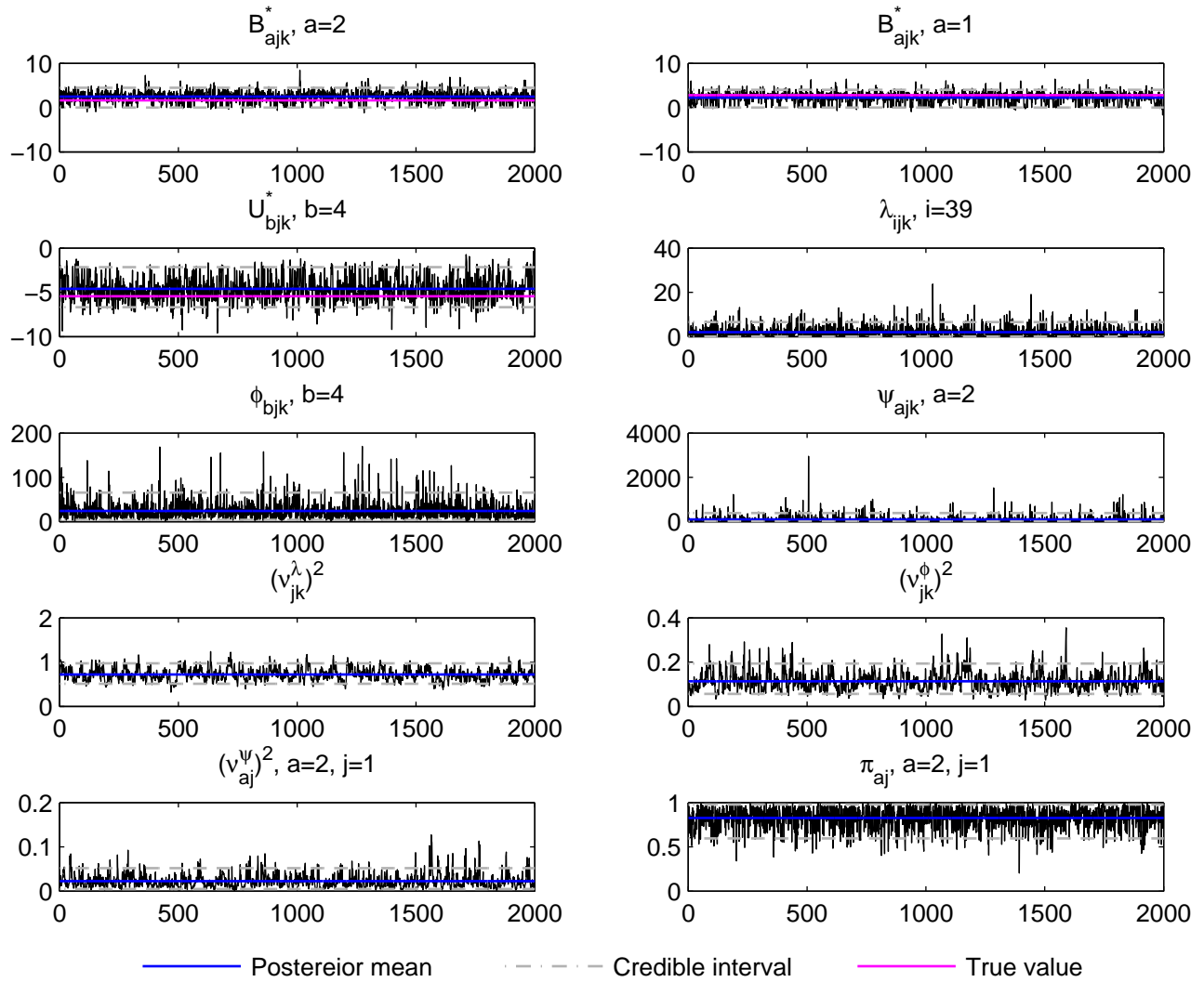
Trace plot, j=1, k=3, t_j data, simulation run 9
