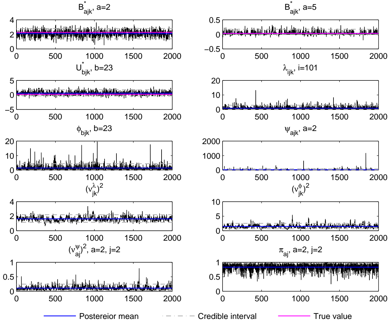
Trace plot, j=2, k=6, t_3 data, simulation run 9
