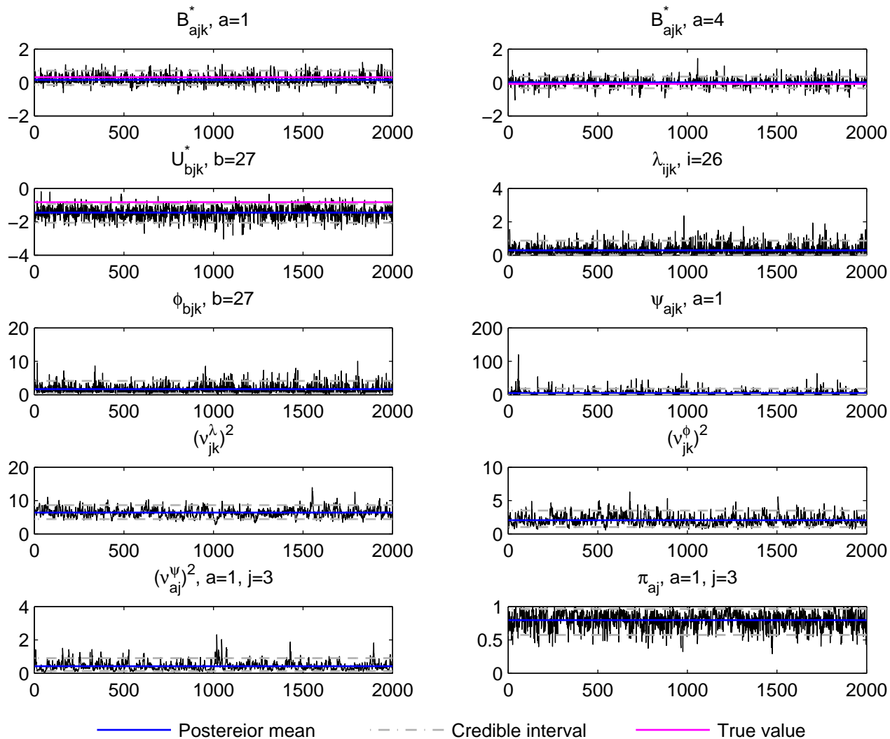
Trace plot, j=3, k=5 , DE data, simulation run 9
