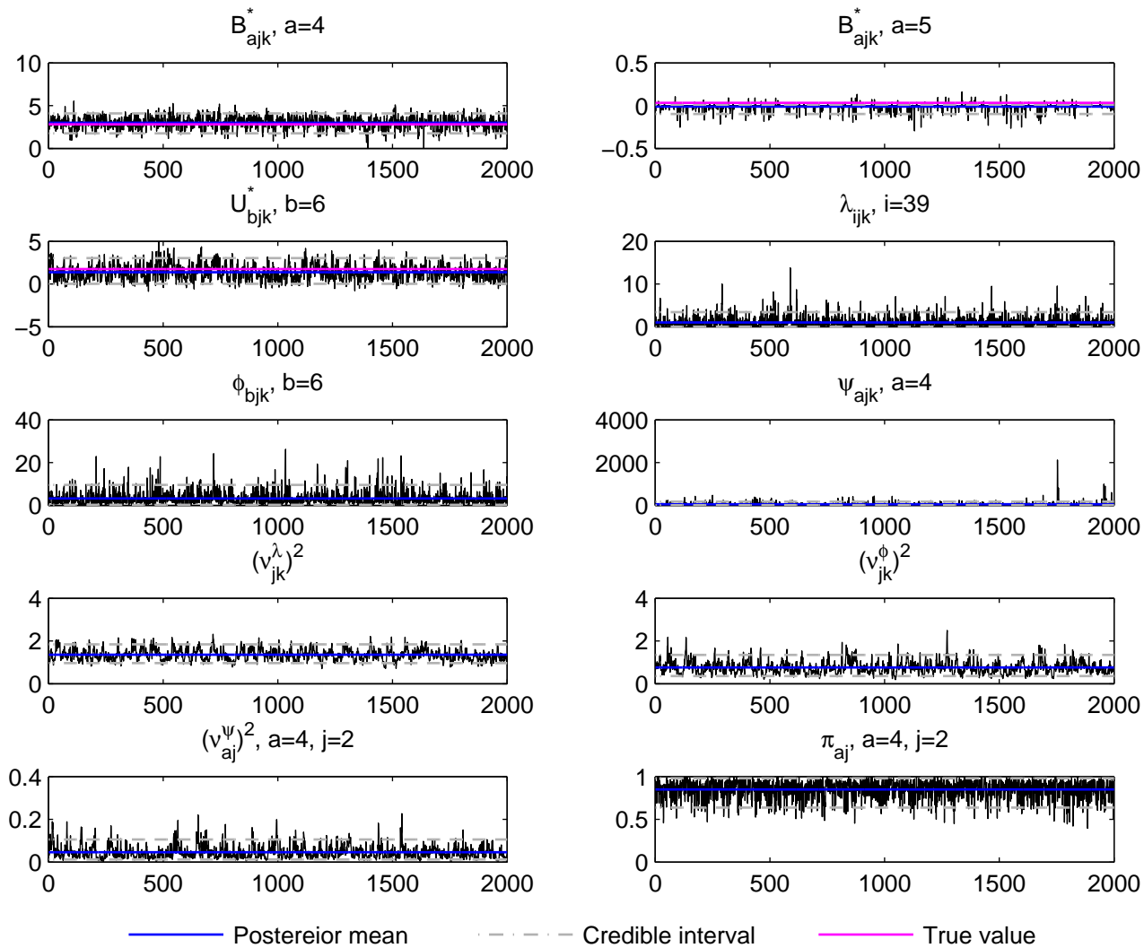
Trace plot, j=2, k=6 , Normal data, simulation run 9
