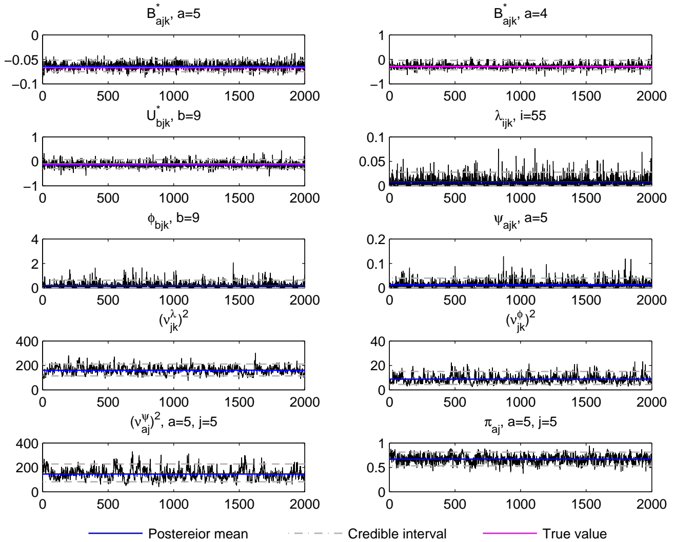
Trace plot, j=5, k=1, t_j data, simulation run 9
