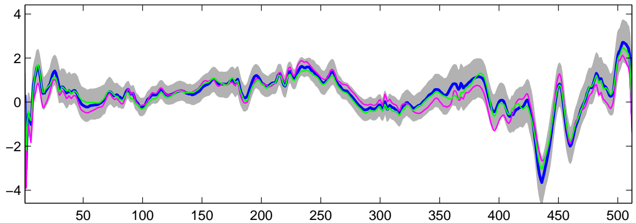
Estimated U_{10}(t) using R-WFMM: DE data, run 9
