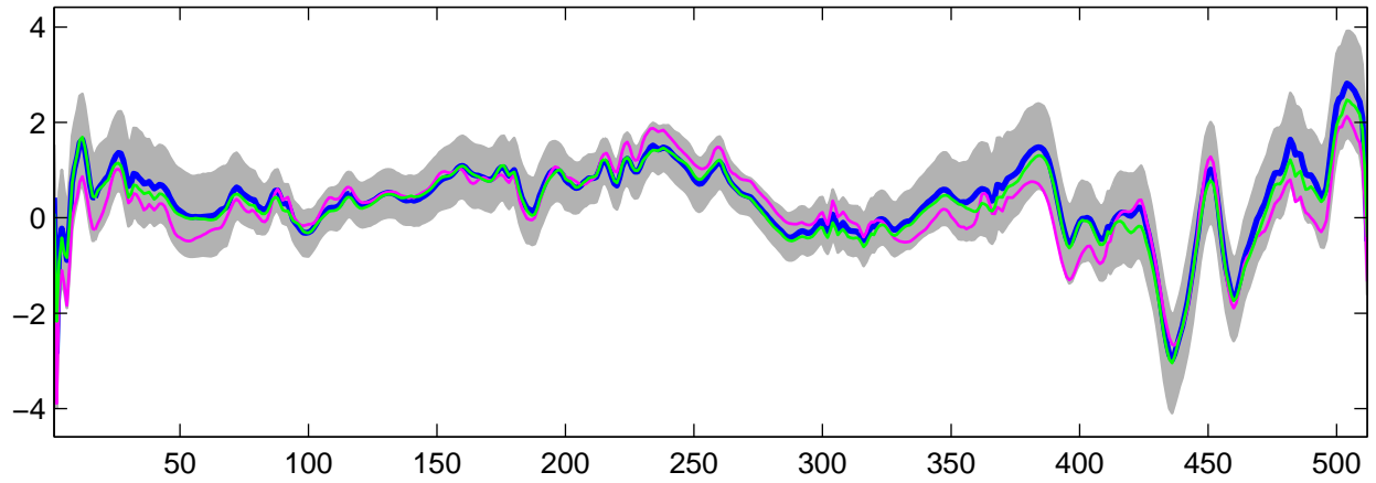
Estimated U_{10}(t) using G-WFMM: DE data, run 9
