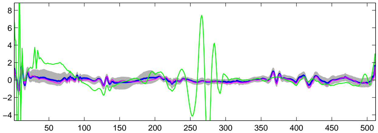
Estimated U_{10}(t) using R-WFMM: t_1 data, run 9
