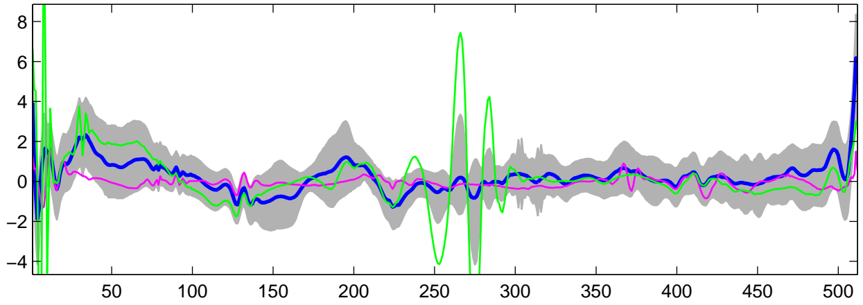
Estimated U_{10}(t) using G-WFMM: t_1 data, run 9
