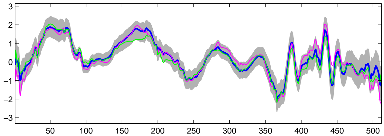
Estimated U_{10}(t) using R-WFMM: t_3 data, run 9
