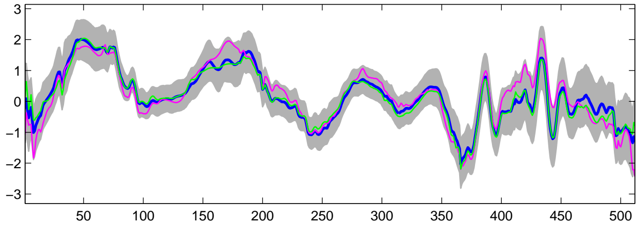
Estimated U_{10}(t) using G-WFMM: t_3 data, run 9
