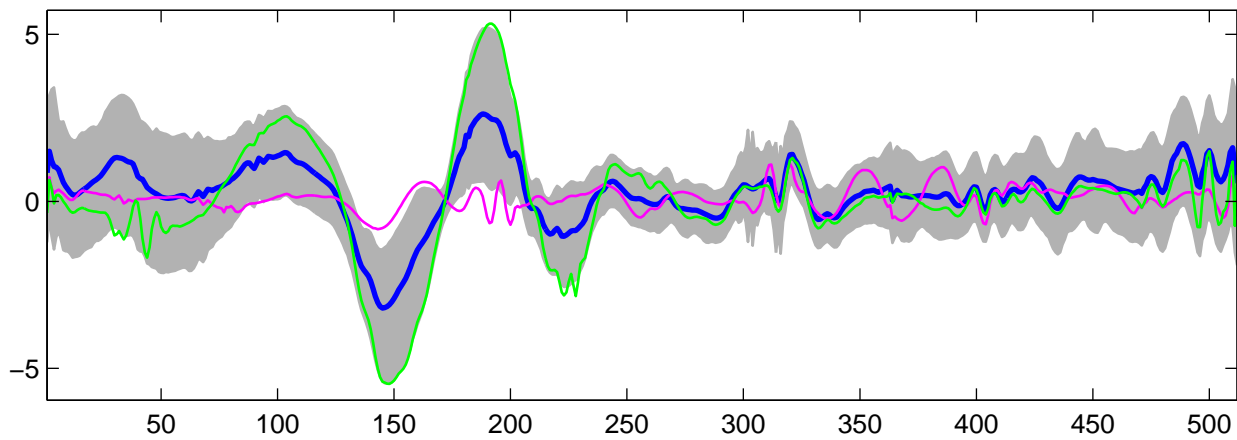
Estimated U_{11}(t) using G-WFMM: t_1 data, run 9
