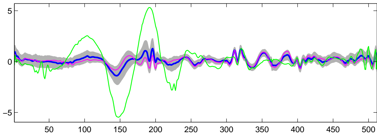
Estimated U_{11}(t) using R-WFMM: t_1 data, run 9
