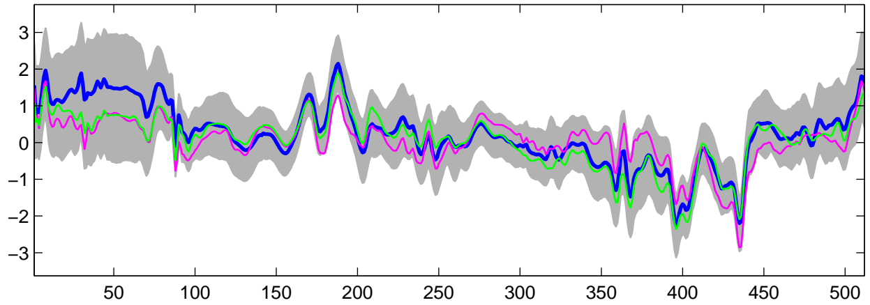
Estimated U_{11}(t) using G-WFMM: t_2 data, run 9
