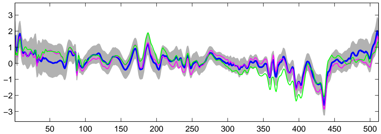
Estimated U_{11}(t) using R-WFMM: t_2 data, run 9
