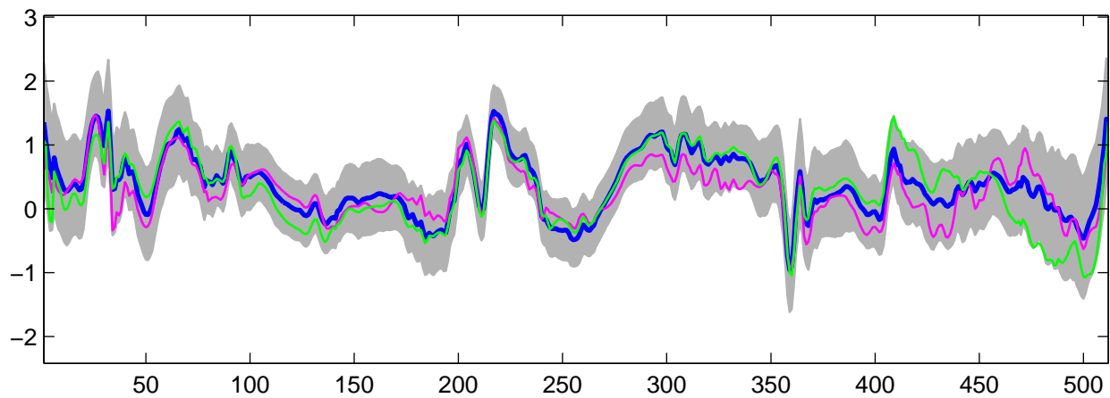
Estimated U_{12}(t) using R-WFMM: DE data, run 9
