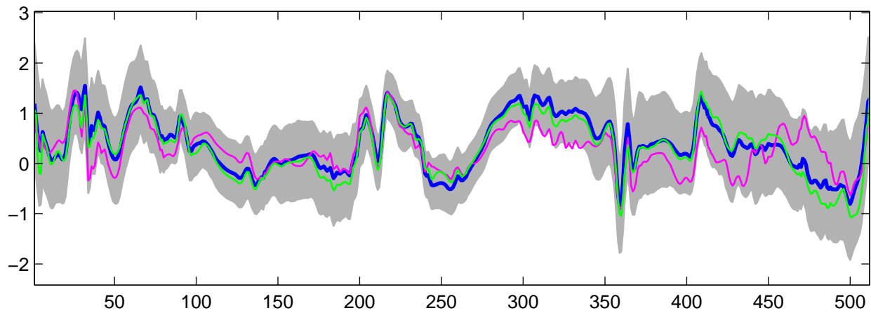
Estimated U_{12}(t) using G-WFMM: DE data, run 9
