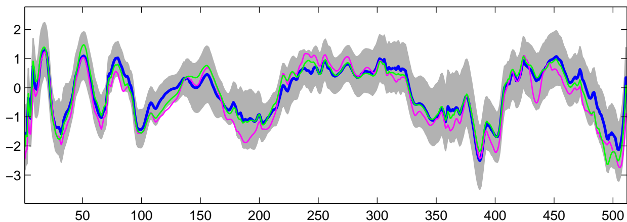
Estimated U_{12}(t) using R-WFMM: Normal data, run 9
