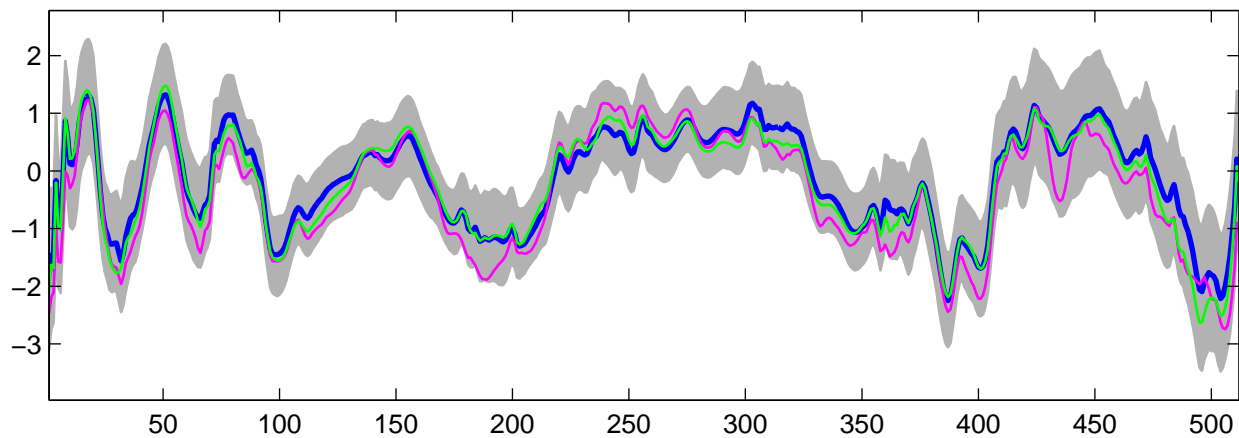
Estimated U_{12}(t) using G-WFMM: Normal data, run 9
