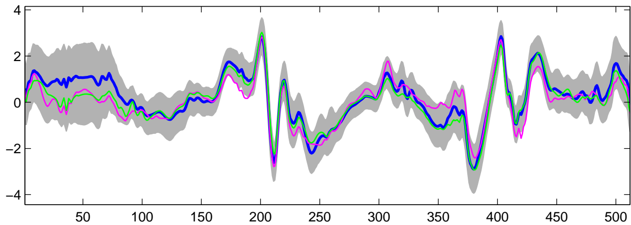
Estimated U_{12}(t) using G-WFMM: t_2 data, run 9
