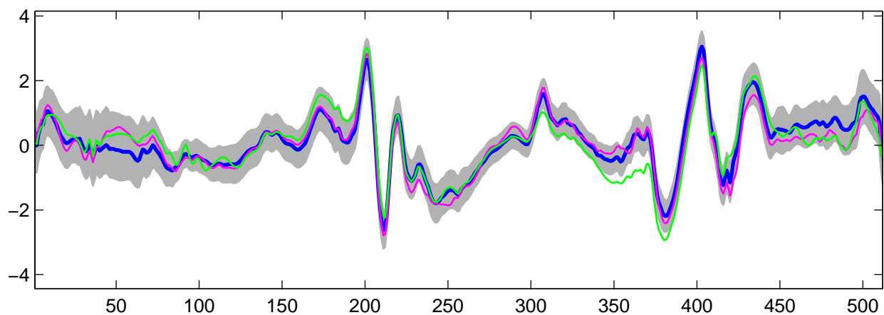
Estimated U_{12}(t) using R-WFMM: t_2 data, run 9
