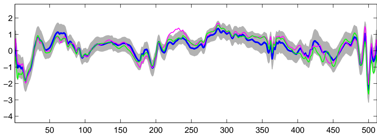
Estimated U_{12}(t) using R-WFMM: t_3 data, run 9
