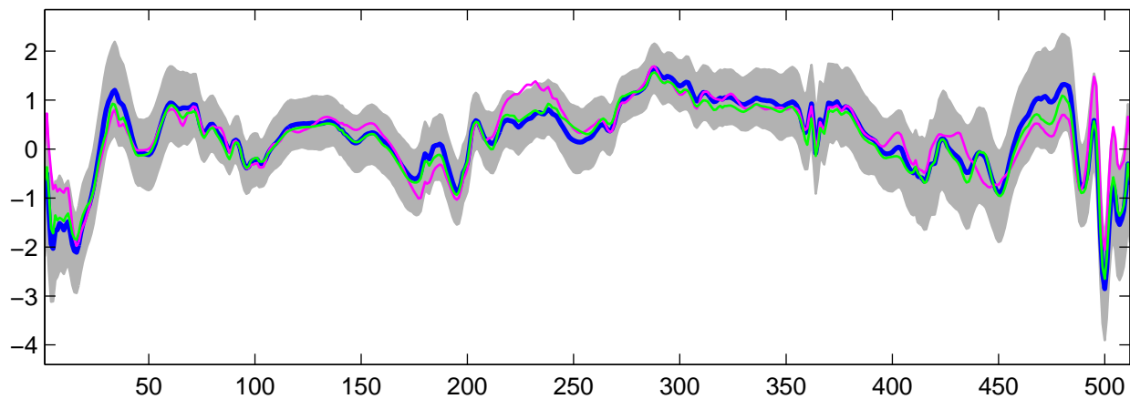
Estimated U_{12}(t) using G-WFMM: t_3 data, run 9
