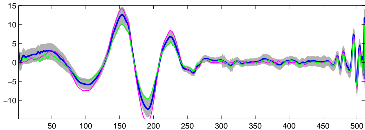
Estimated U_{13}(t) using G-WFMM: t_1 data, run 9
