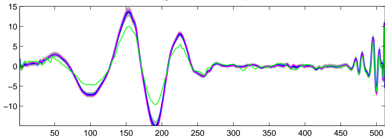
Estimated U_{13}(t) using R-WFMM: t_1 data, run 9
