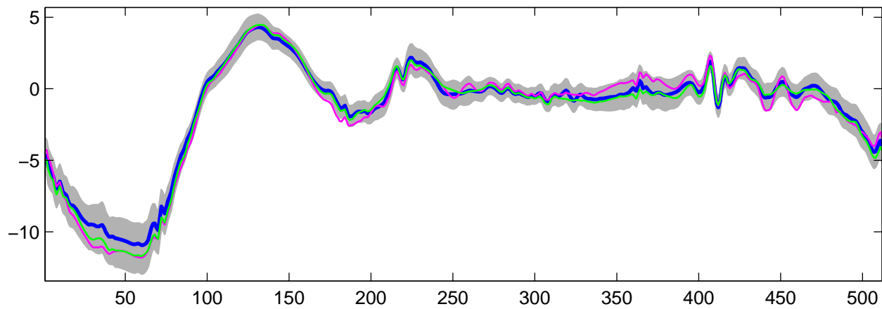
Estimated U_{13}(t) using G-WFMM: t_2 data, run 9
