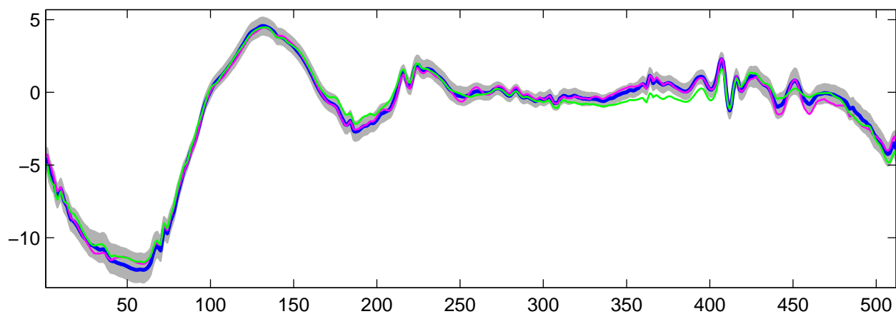
Estimated U_{13}(t) using R-WFMM: t_2 data, run 9
