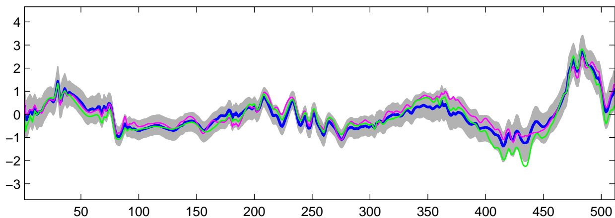
Estimated U_{13}(t) using R-WFMM: t_3 data, run 9
