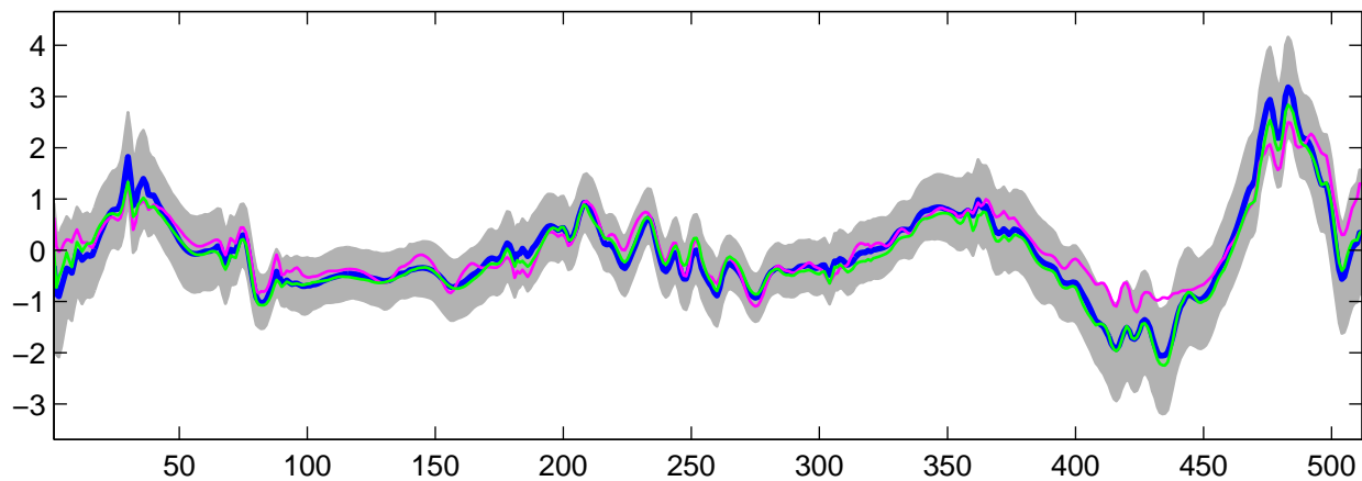
Estimated U_{13}(t) using G-WFMM: t_3 data, run 9
