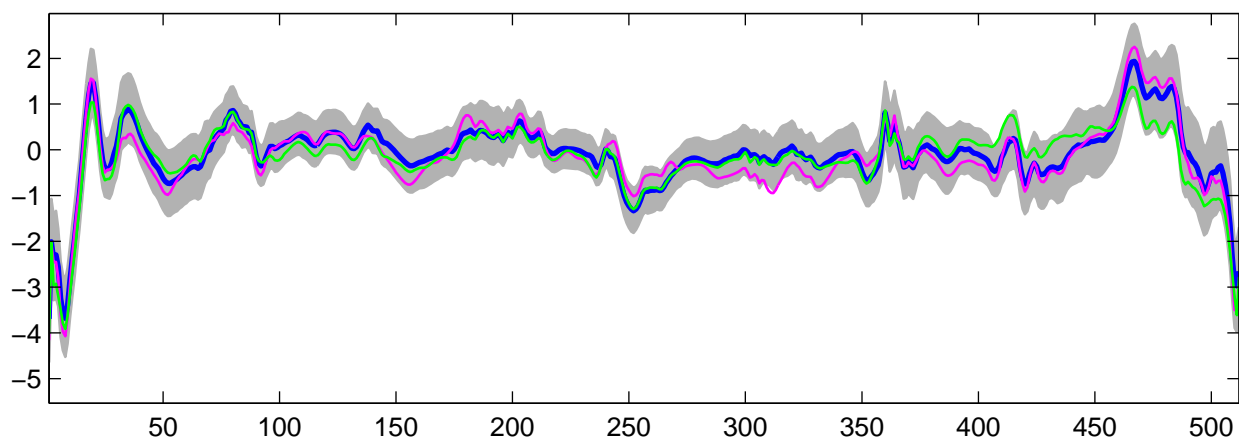
Estimated U_{14}(t) using R-WFMM: DE data, run 9
