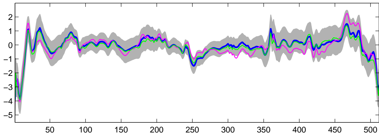
Estimated U_{14}(t) using G-WFMM: DE data, run 9
