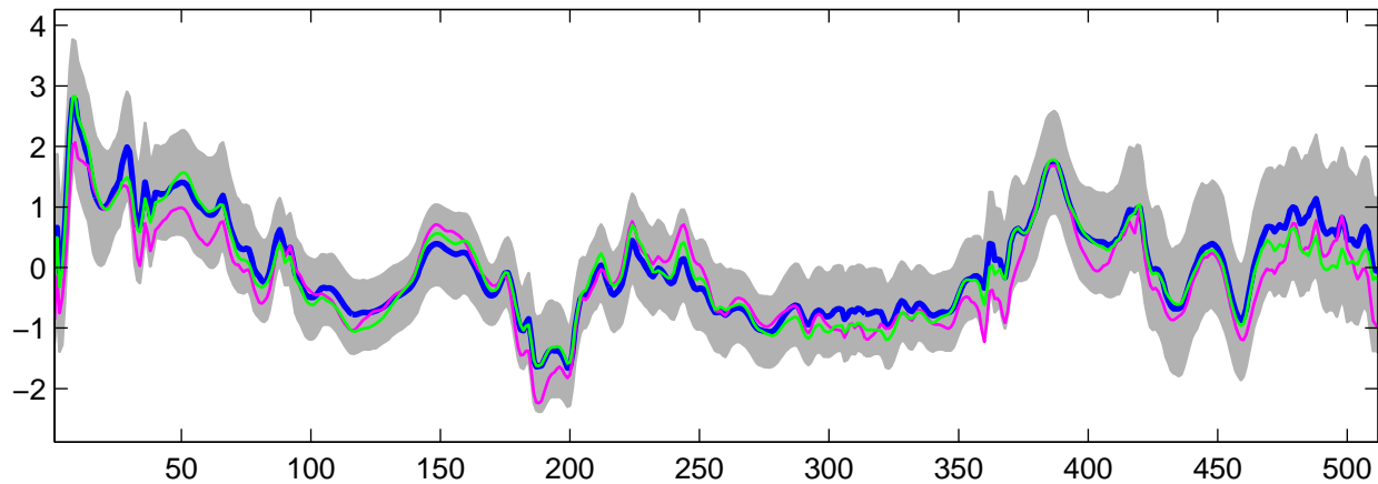
Estimated U_{14}(t) using G-WFMM: Normal data, run 9
