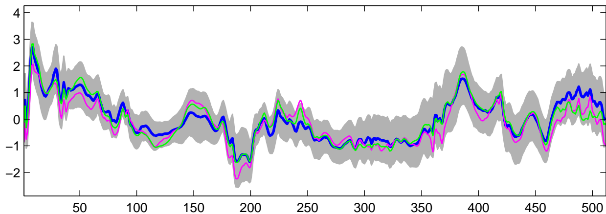
Estimated U_{14}(t) using R-WFMM: Normal data, run 9
