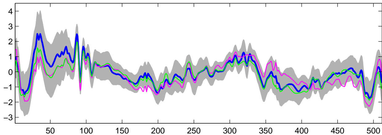
Estimated U_{14}(t) using G-WFMM: t_2 data, run 9
