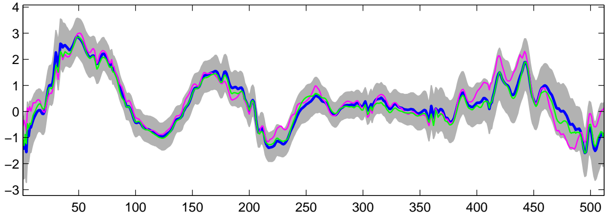
Estimated U_{14}(t) using G-WFMM: t_3 data, run 9
