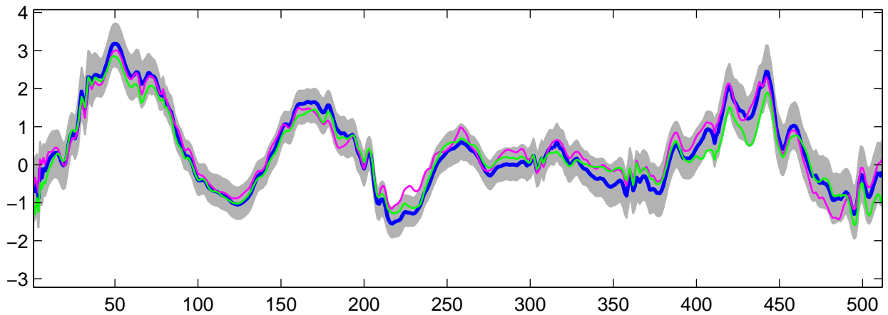
Estimated U_{14}(t) using R-WFMM: t_3 data, run 9
